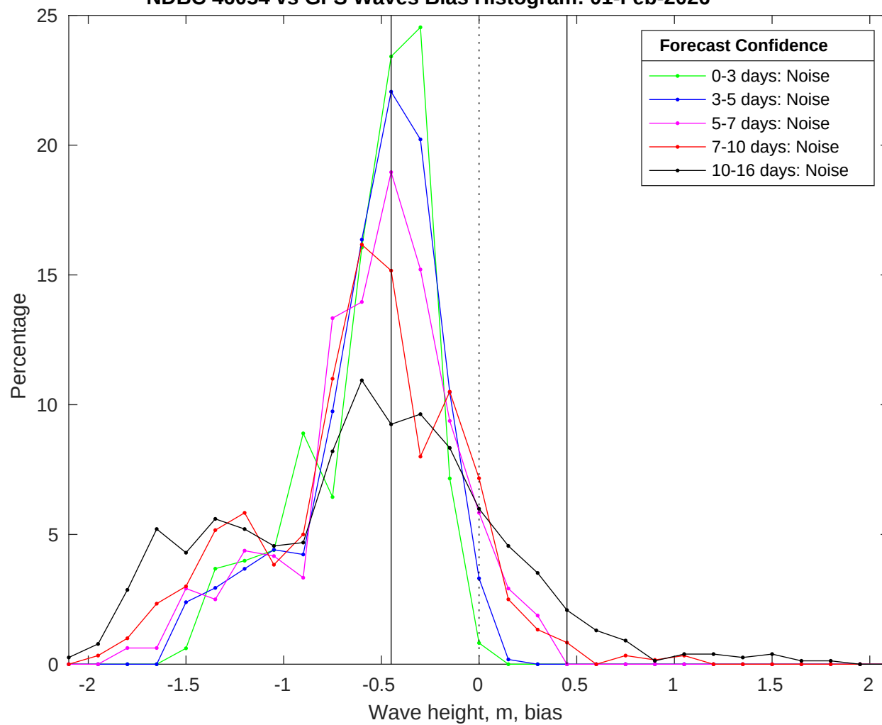
NDBC 46054 vs GFS Waves Bias Histogram: 01-Feb-2026
