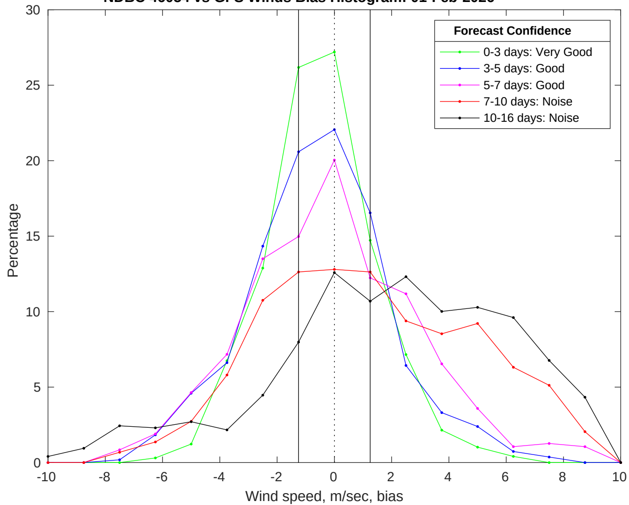
NDBC 46054 vs GFS Winds Bias Histogram: 01-Feb-2026
