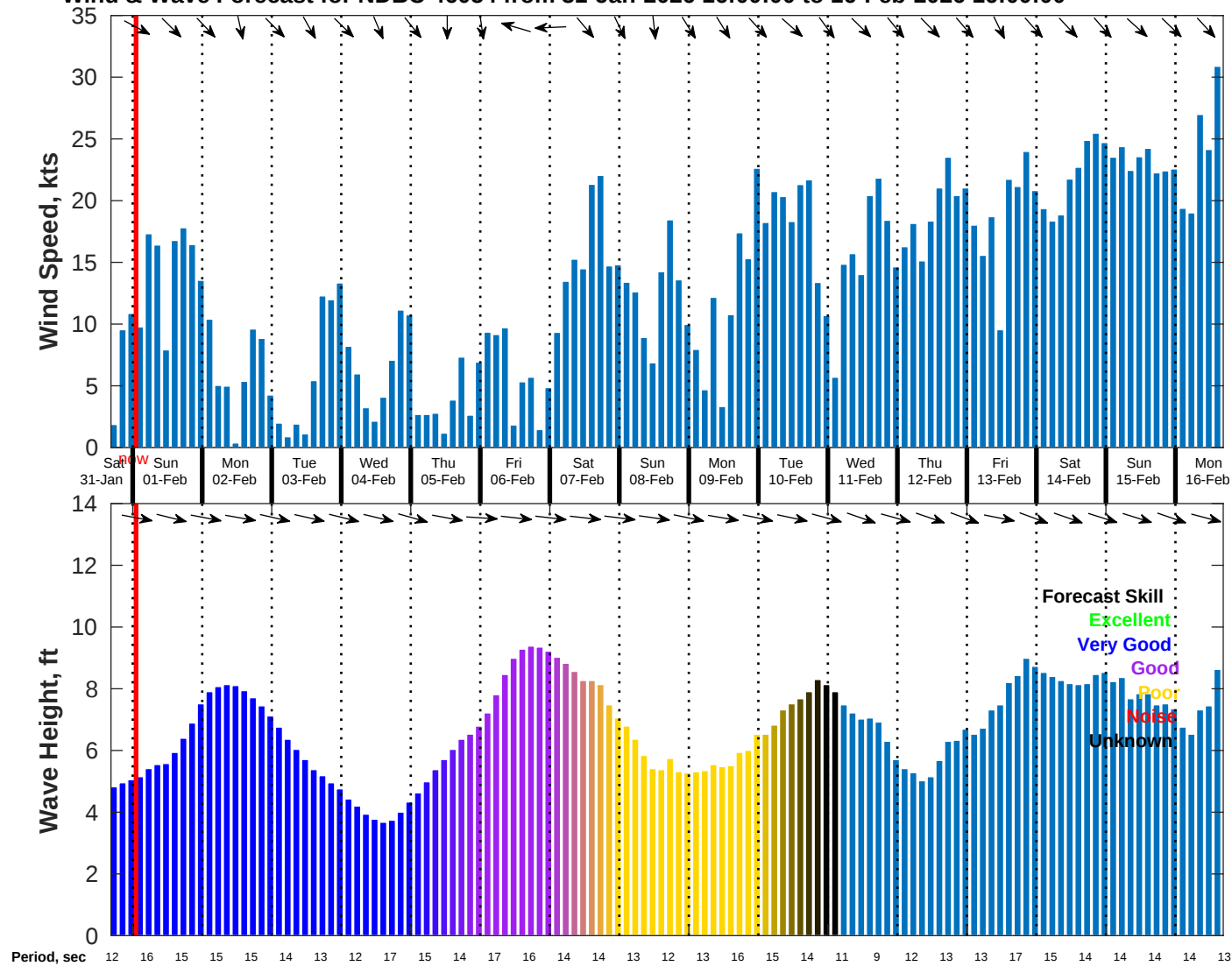
Wind & Wave Forecast for NDBC 46054 from 31-Jan-2026 16:00:00 to 16-Feb-2026 16:00:00
