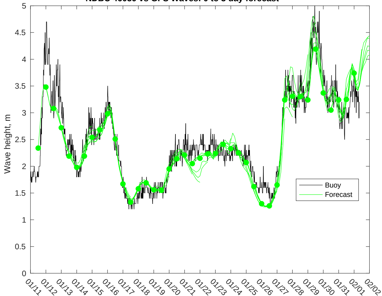
NDBC 46059 vs GFS Waves: 0 to 3 day forecast
