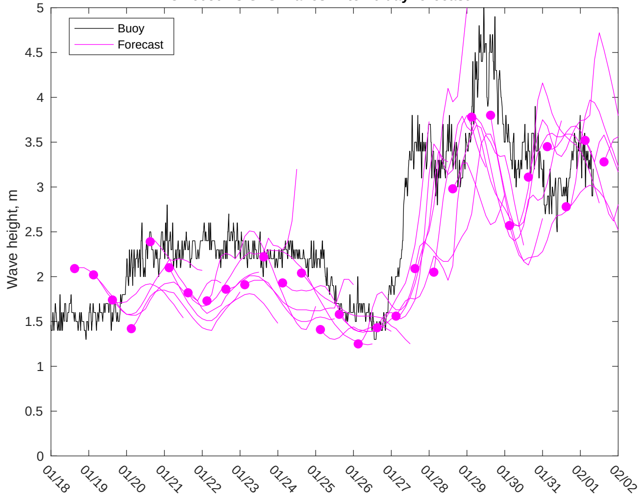
NDBC 46059 vs GFS Waves: 7 to 10 day forecast
