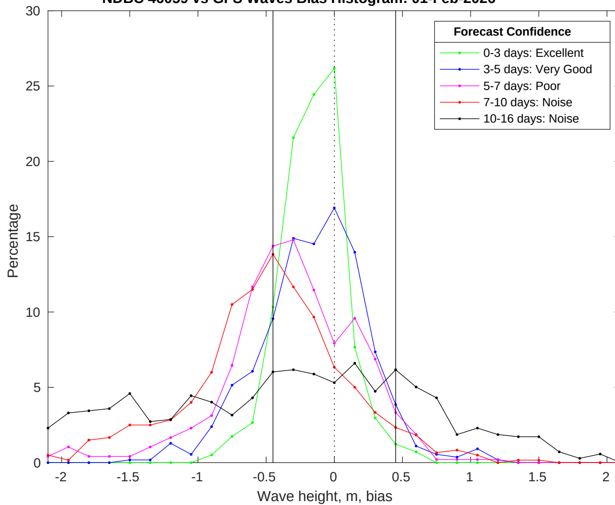
NDBC 46059 vs GFS Waves Bias Histogram: 01-Feb-2026
