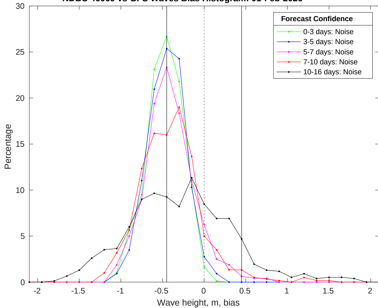
NDBC 46069 vs GFS Waves Bias Histogram: 01-Feb-2026
