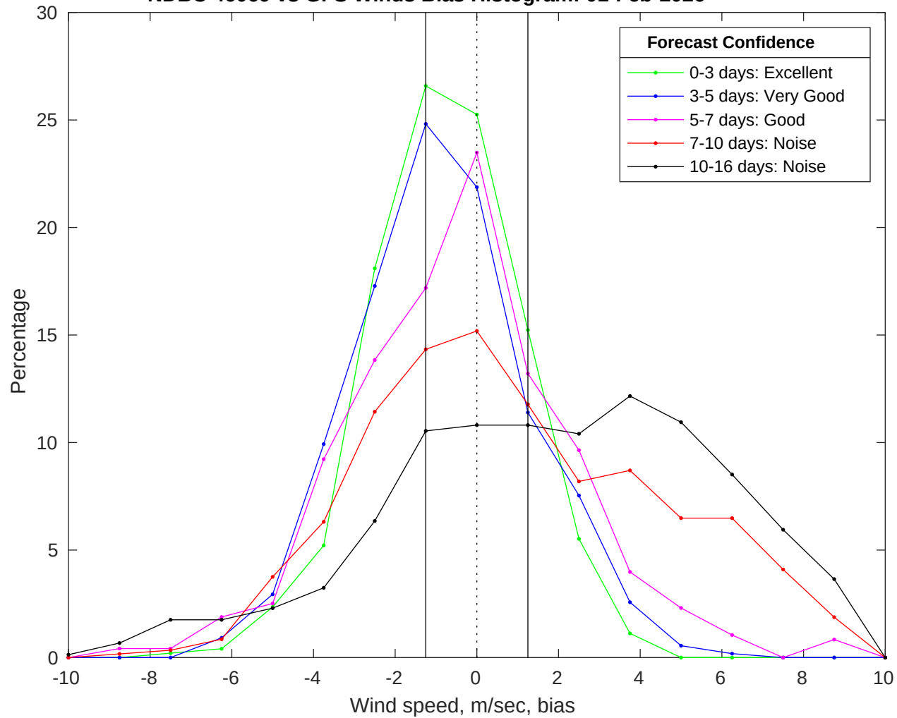
NDBC 46069 vs GFS Winds Bias Histogram: 01-Feb-2026
