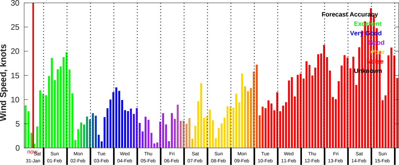
GFS Wind Speed Forecast for NDBC 46069 from 31-Jan-2026 04:00:00 to 16-Feb-2026 04:00:00
