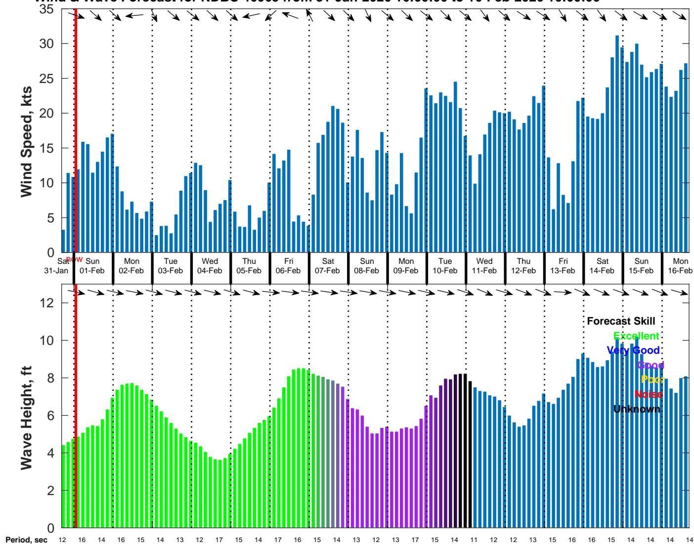
Wind & Wave Forecast for NDBC 46069 from 31-Jan-2026 16:00:00 to 16-Feb-2026 16:00:00
