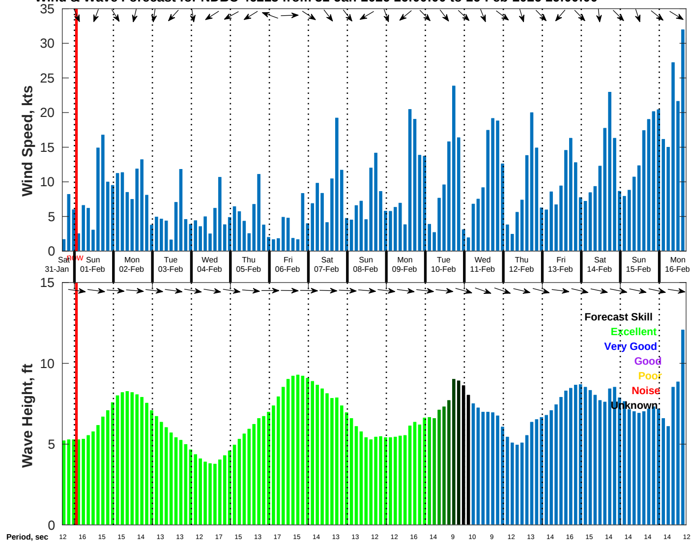
Wind & Wave Forecast for NDBC 46215 from 31-Jan-2026 16:00:00 to 16-Feb-2026 16:00:00
