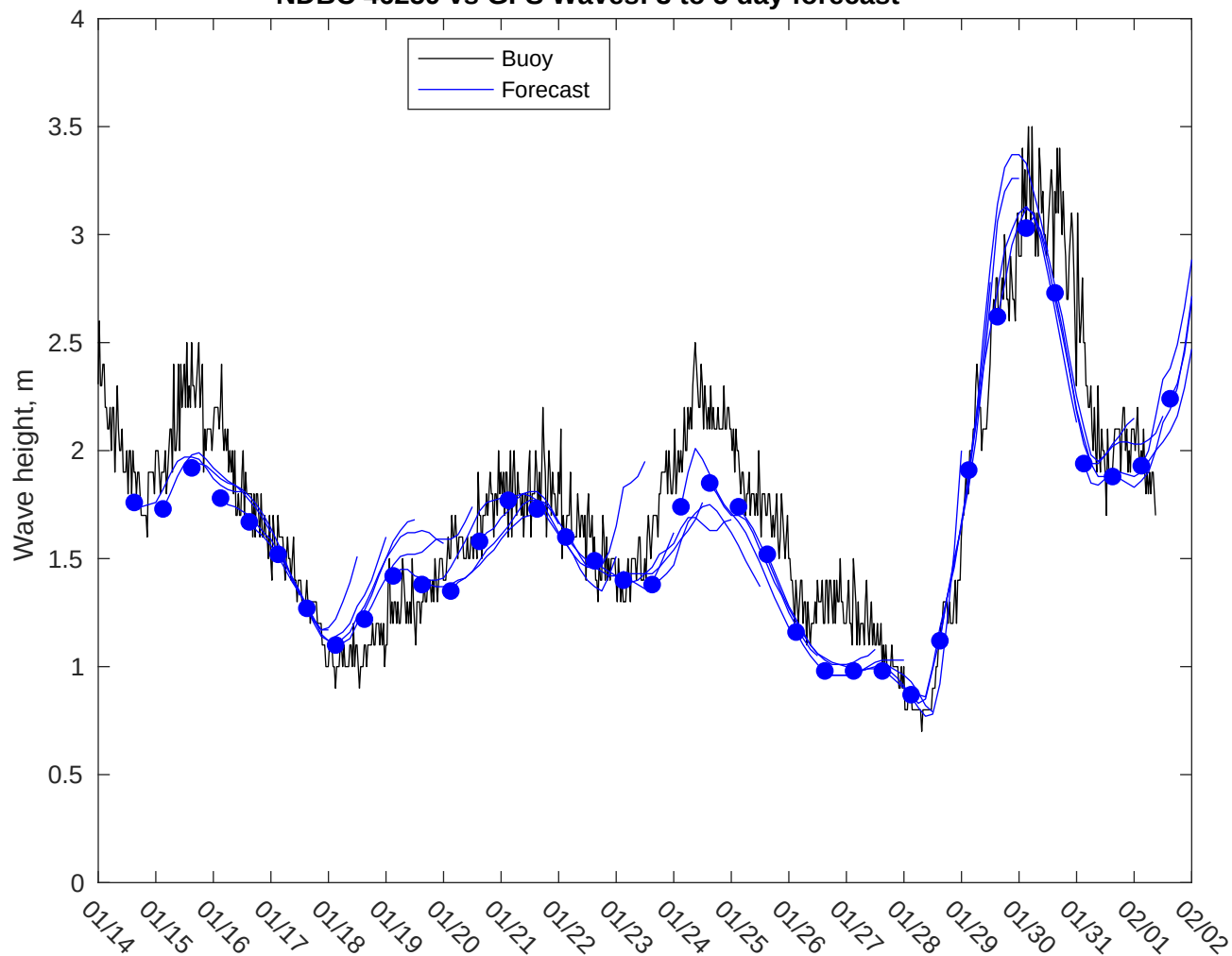
NDBC 46259 vs GFS Waves: 3 to 5 day forecast
