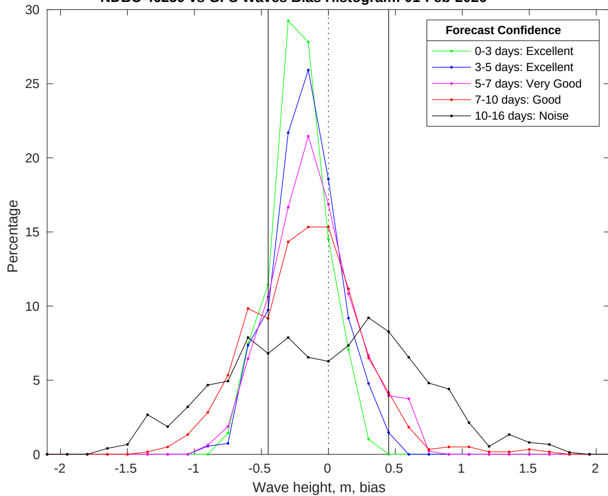
NDBC 46259 vs GFS Waves Bias Histogram: 01-Feb-2026
