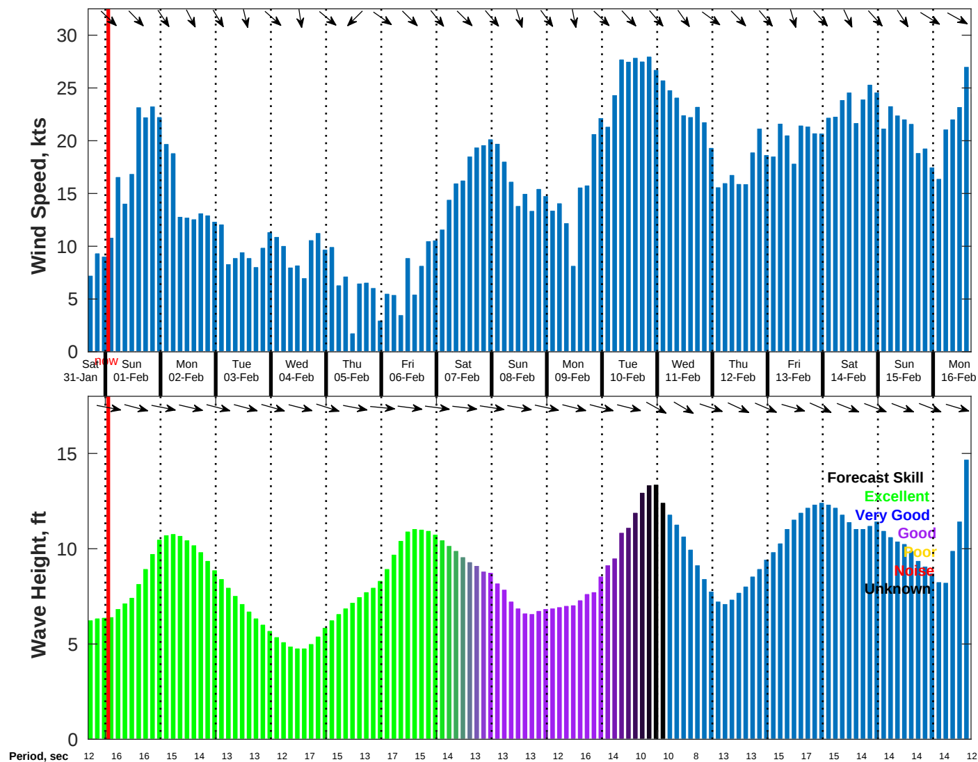
Wind & Wave Forecast for NDBC 46259 from 31-Jan-2026 16:00:00 to 16-Feb-2026 16:00:00
