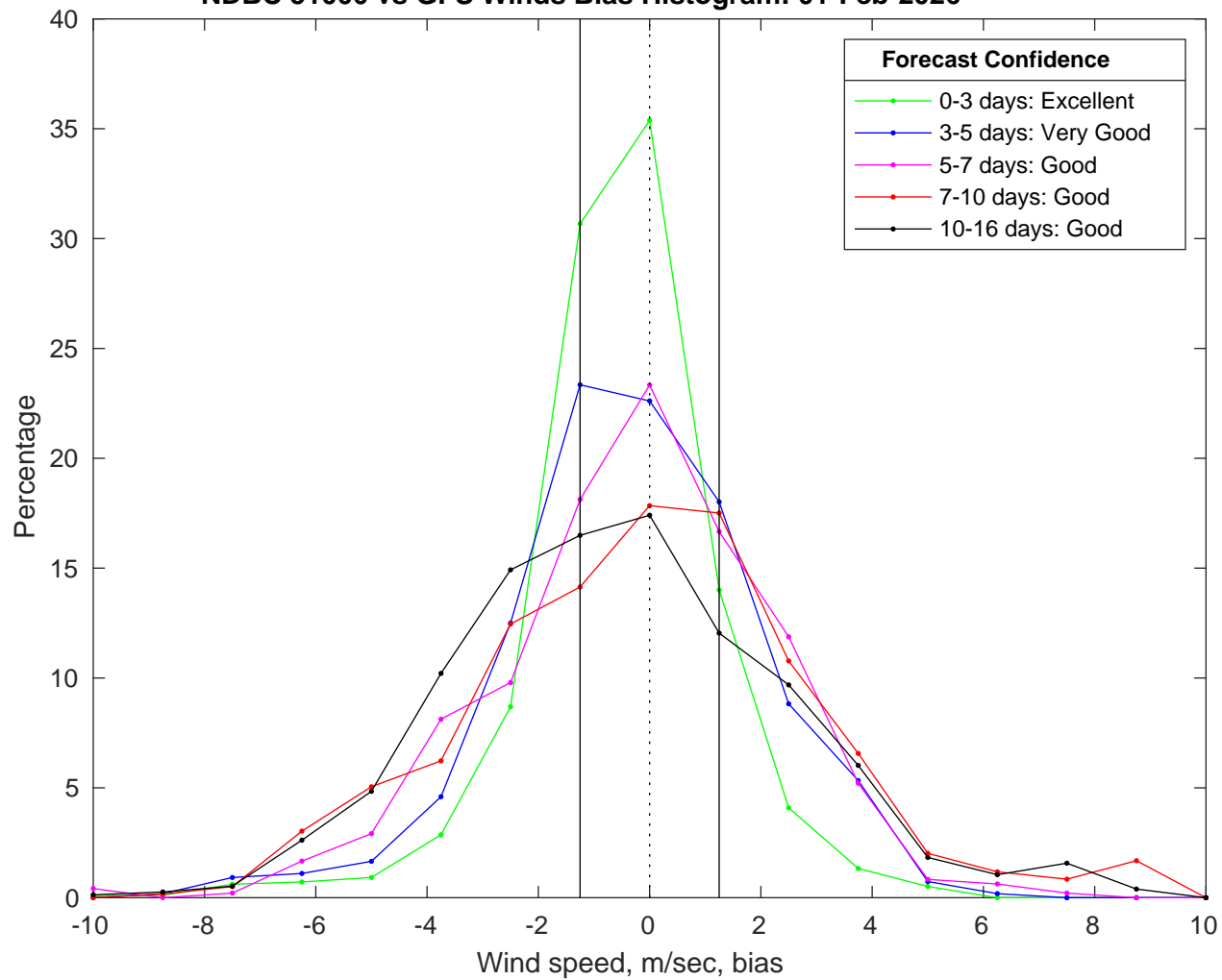
NDBC 51000 vs GFS Winds Bias Histogram: 01-Feb-2026
