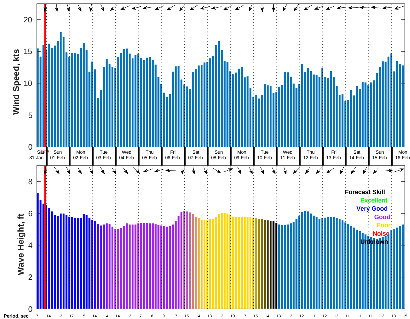
Wind & Wave Forecast for NDBC 51209 from 31-Jan-2026 13:00:00 to 16-Feb-2026 13:00:00
