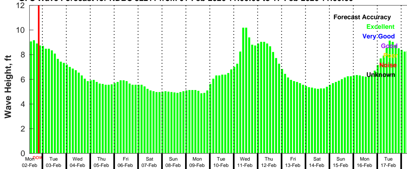
GFS Wave Forecast for NDBC 52211 from 01-Feb-2026 11:00:00 to 17-Feb-2026 11:00:00
