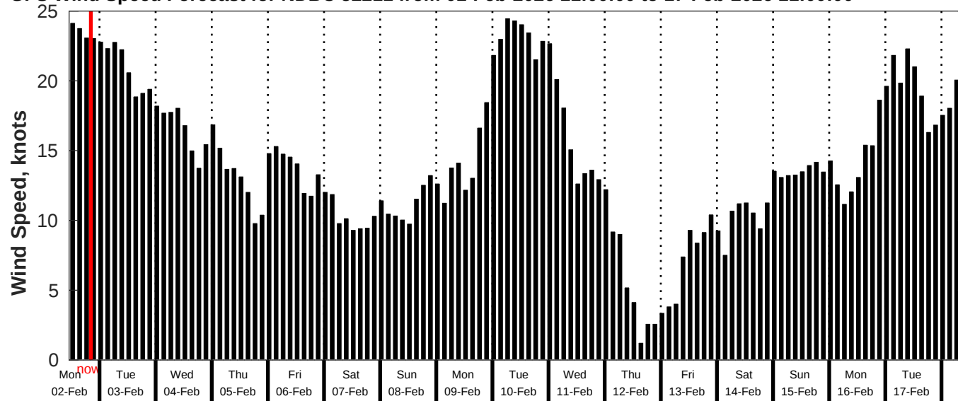
GFS Wind Speed Forecast for NDBC 52211 from 01-Feb-2026 11:00:00 to 17-Feb-2026 11:00:00
