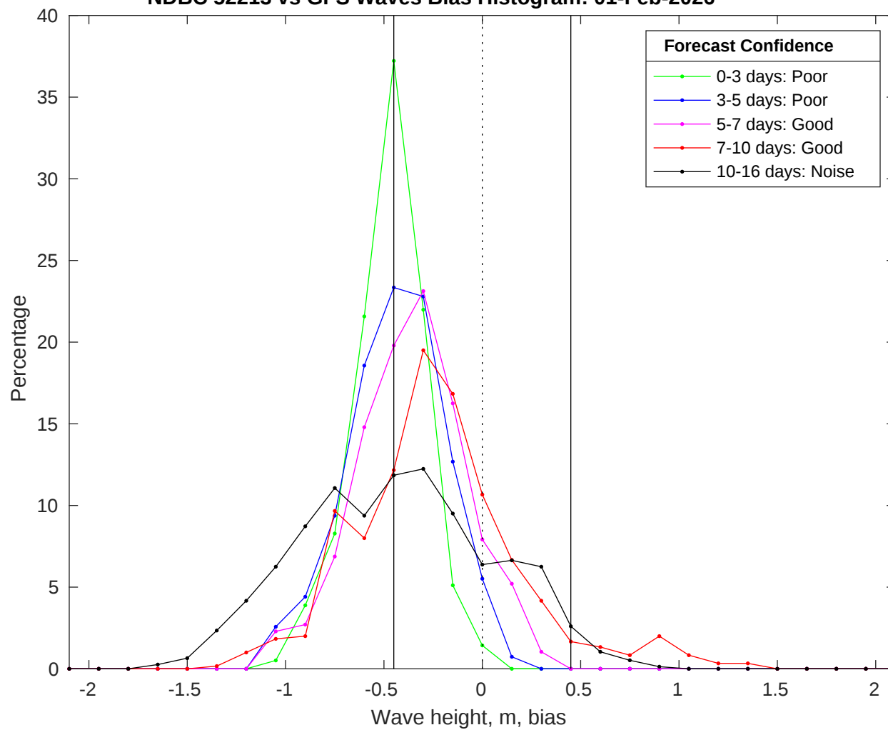
NDBC 52213 vs GFS Waves Bias Histogram: 01-Feb-2026
