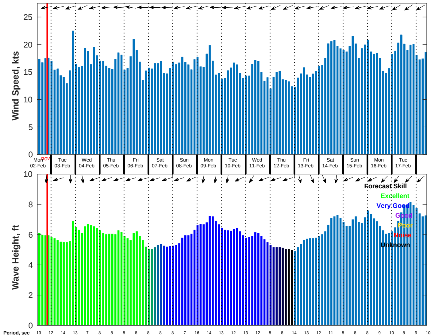
Wind & Wave Forecast for NDBC 52213 from 01-Feb-2026 11:00:00 to 17-Feb-2026 11:00:00
