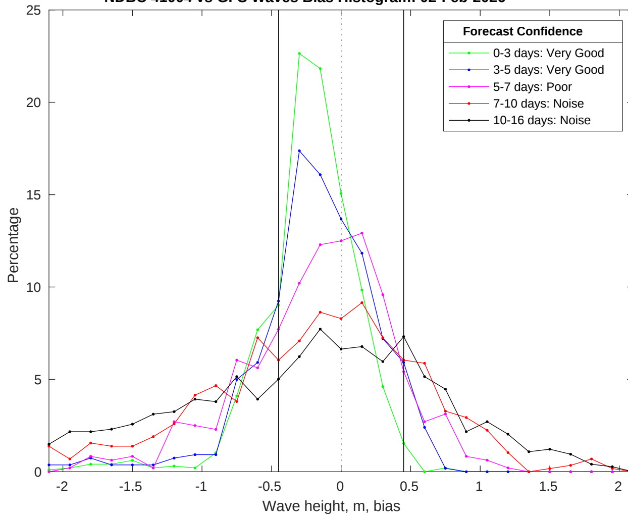
NDBC 41004 vs GFS Waves Bias Histogram: 02-Feb-2026
