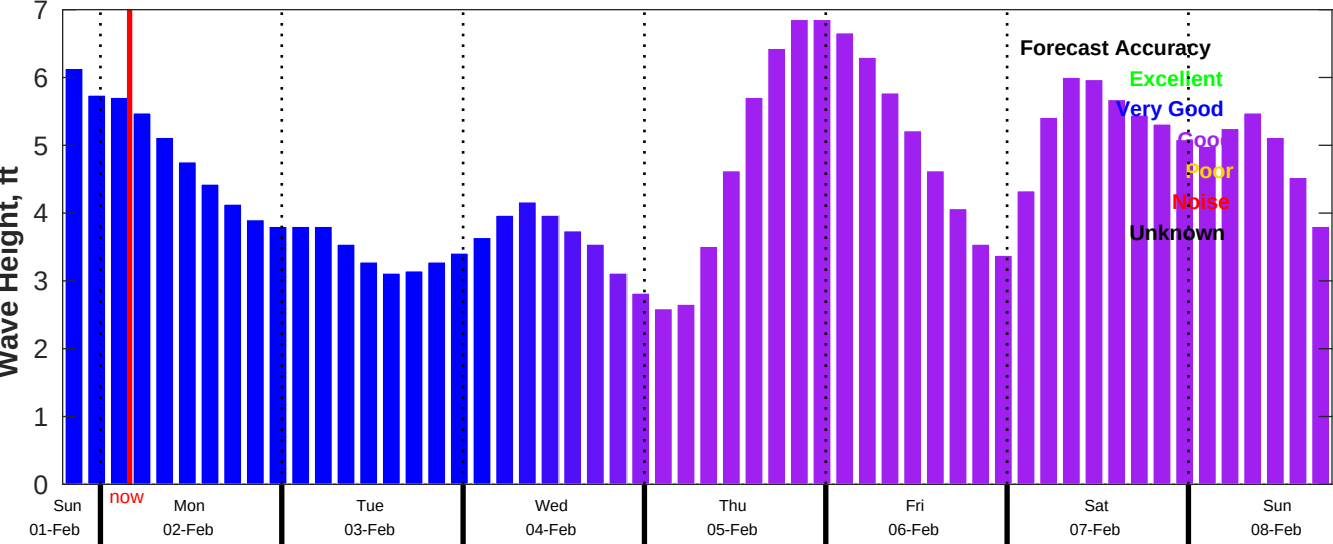
CMEMS Wave Forecast for NDBC 41004 from 01-Feb-2026 19:00:00 to 08-Feb-2026 19:00:00
