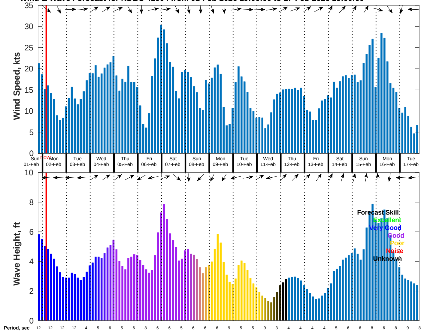
Wind & Wave Forecast for NDBC 41004 from 01-Feb-2026 19:00:00 to 17-Feb-2026 19:00:00
