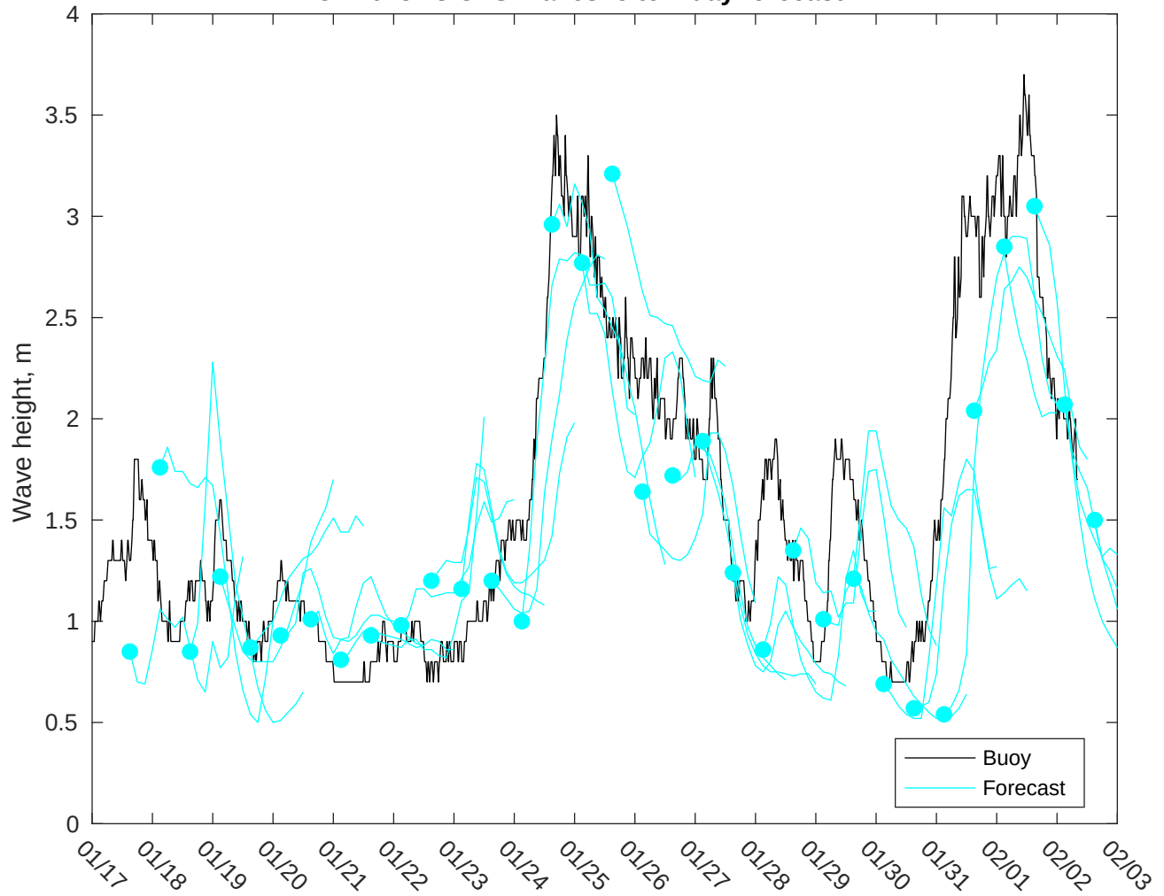
NDBC 41013 vs GFS Waves: 5 to 7 day forecast
