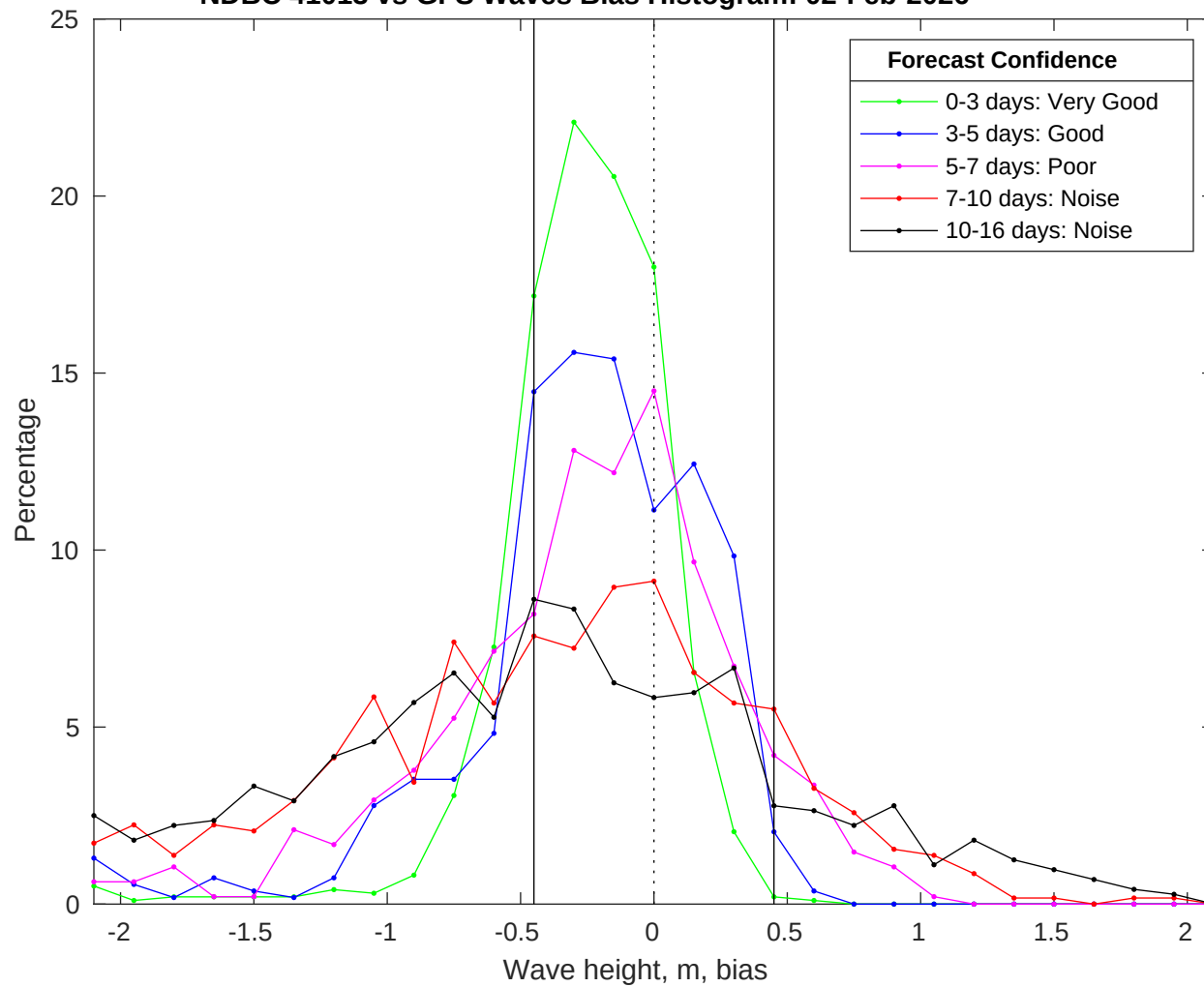
NDBC 41013 vs GFS Waves Bias Histogram: 02-Feb-2026
