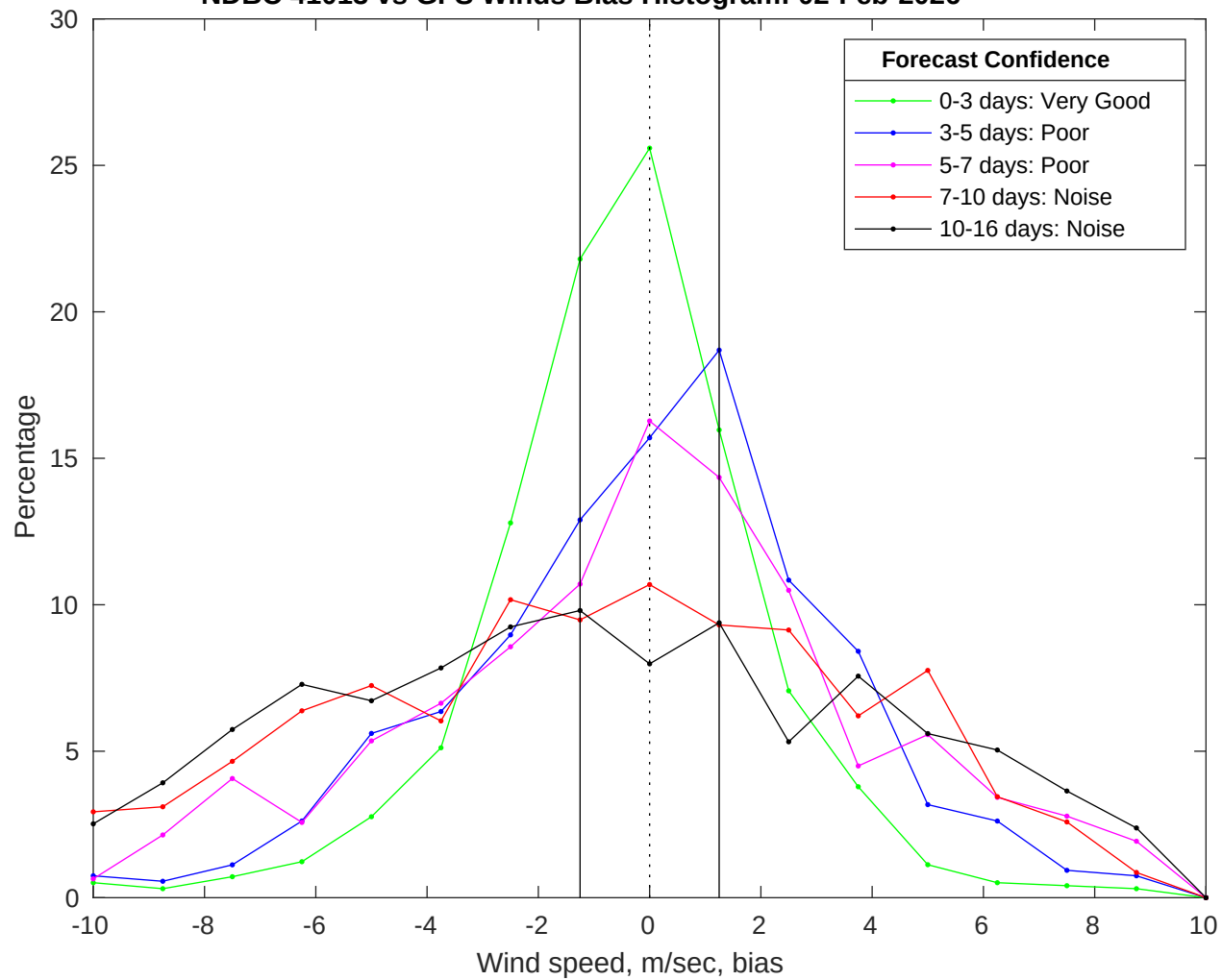
NDBC 41013 vs GFS Winds Bias Histogram: 02-Feb-2026
