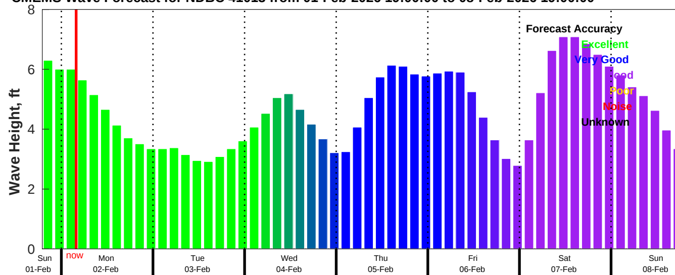
CMEMS Wave Forecast for NDBC 41013 from 01-Feb-2026 19:00:00 to 08-Feb-2026 19:00:00
