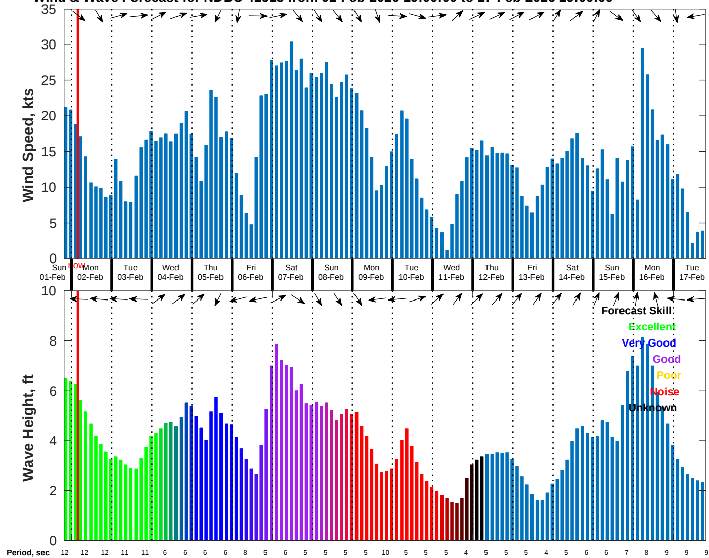
Wind & Wave Forecast for NDBC 41013 from 01-Feb-2026 19:00:00 to 17-Feb-2026 19:00:00
