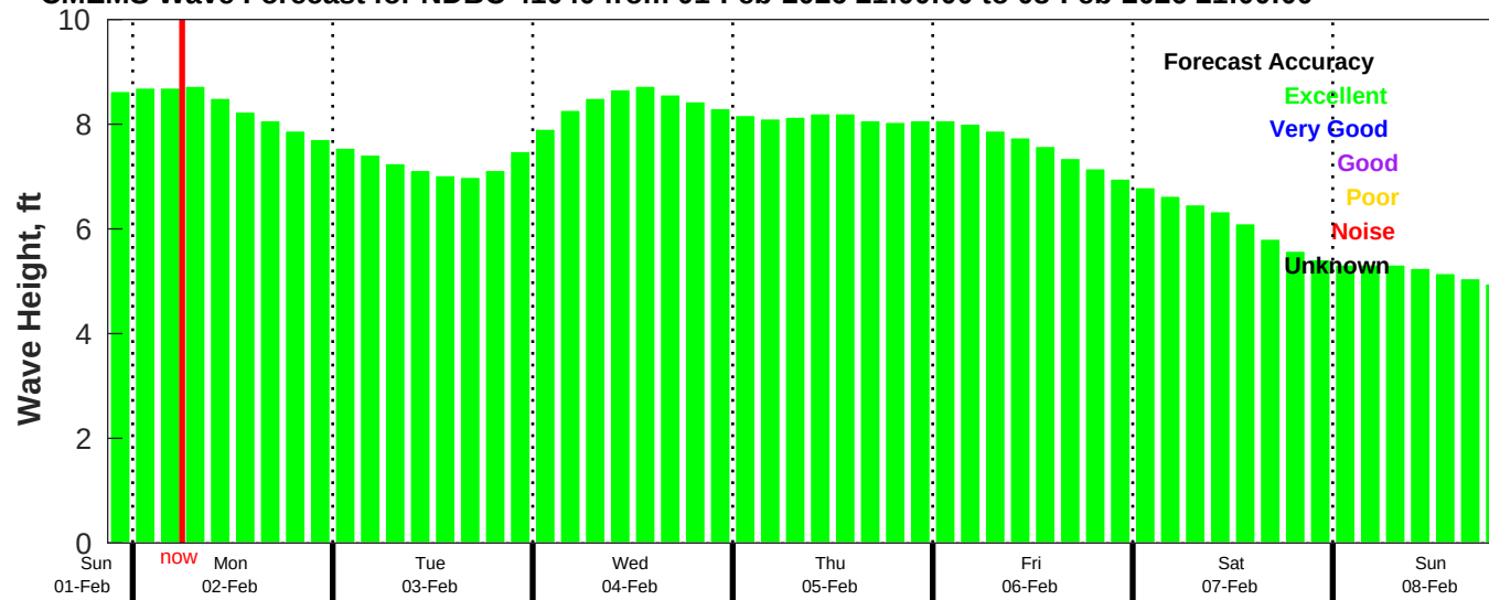
CMEMS Wave Forecast for NDBC 41040 from 01-Feb-2026 21:00:00 to 08-Feb-2026 21:00:00
