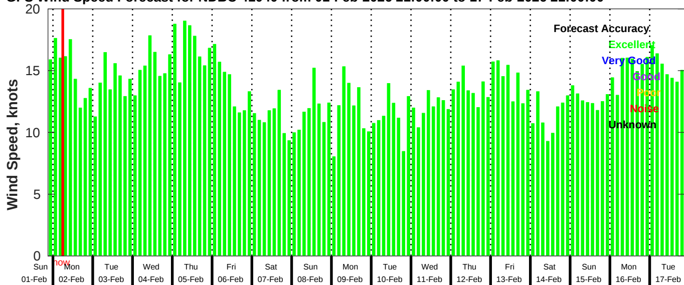
GFS Wind Speed Forecast for NDBC 41040 from 01-Feb-2026 21:00:00 to 17-Feb-2026 21:00:00
