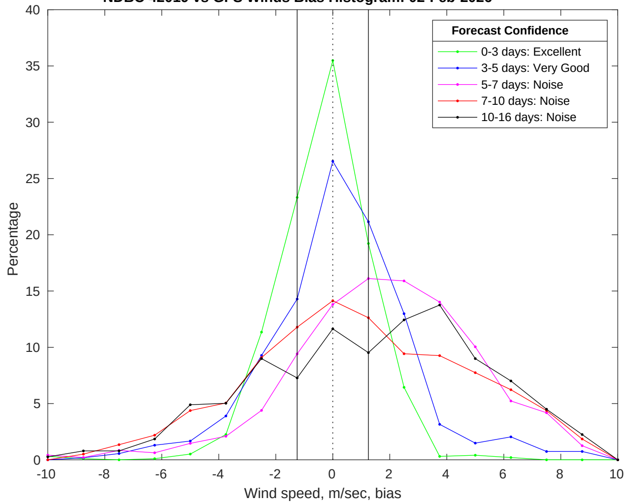
NDBC 42019 vs GFS Winds Bias Histogram: 02-Feb-2026
