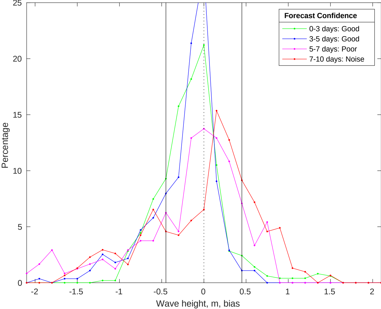
NDBC 42020 vs CMEMS Waves Bias Histogram: 31-Jan-2026
