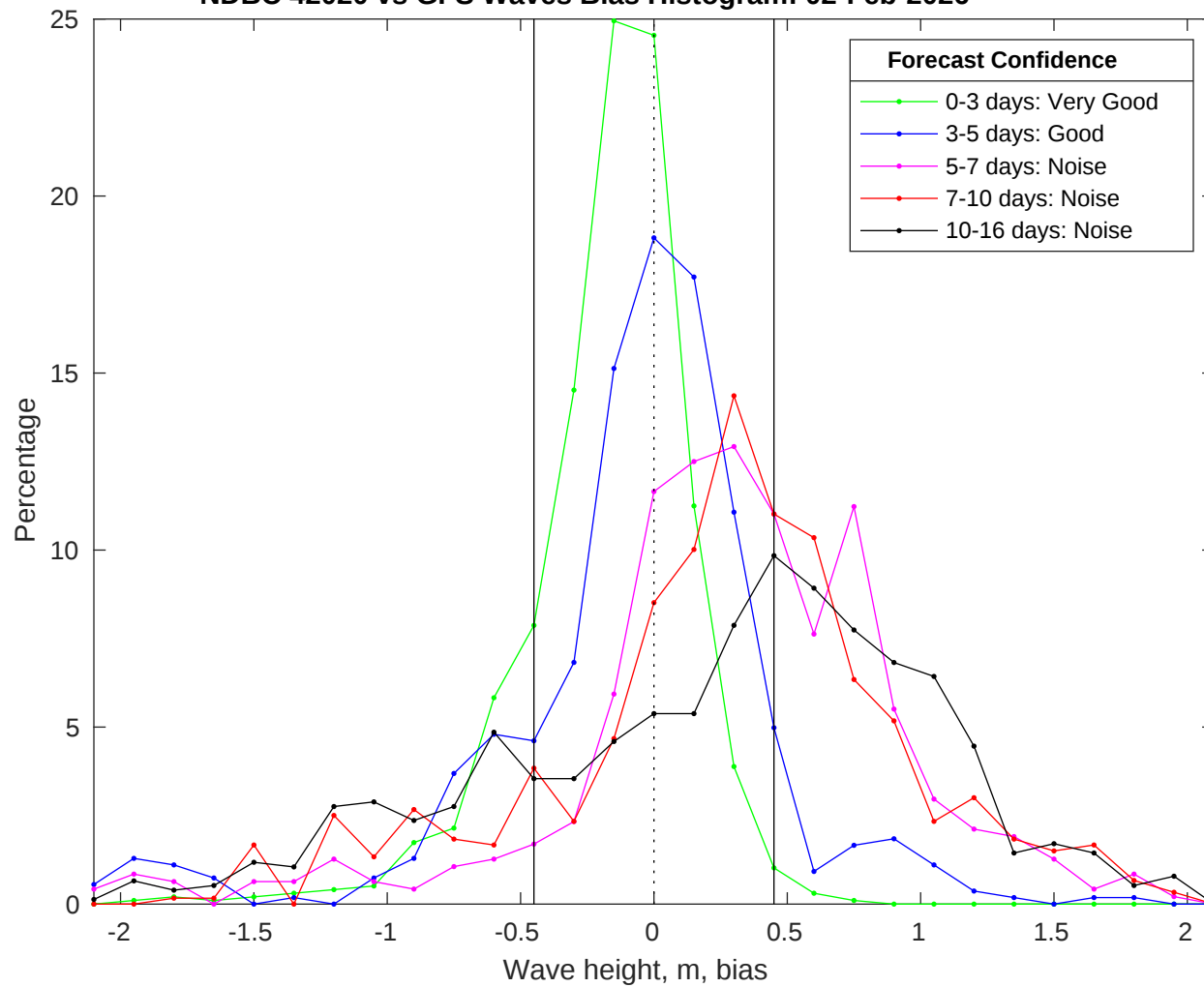
NDBC 42020 vs GFS Waves Bias Histogram: 02-Feb-2026
