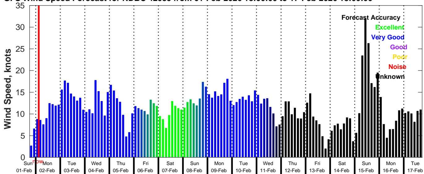
GFS Wind Speed Forecast for NDBC 42035 from 01-Feb-2026 18:00:00 to 17-Feb-2026 18:00:00
