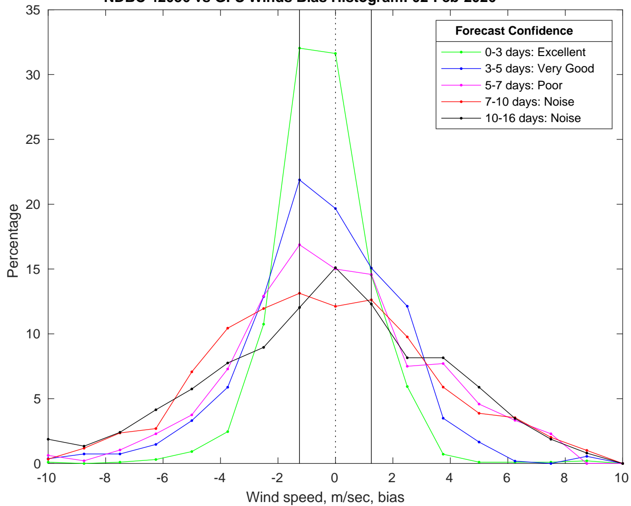
NDBC 42036 vs GFS Winds Bias Histogram: 02-Feb-2026
