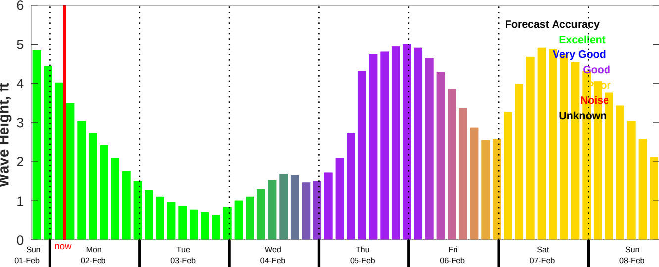
CMEMS Wave Forecast for NDBC 42036 from 01-Feb-2026 19:00:00 to 08-Feb-2026 19:00:00
