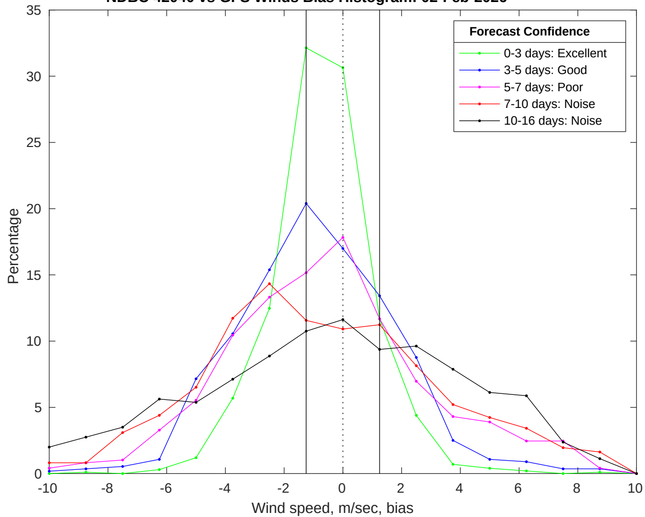
NDBC 42040 vs GFS Winds Bias Histogram: 02-Feb-2026
