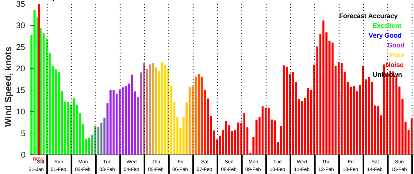
GFS Wind Speed Forecast for NDBC 42040 from 31-Jan-2026 07:00:00 to 16-Feb-2026 07:00:00
