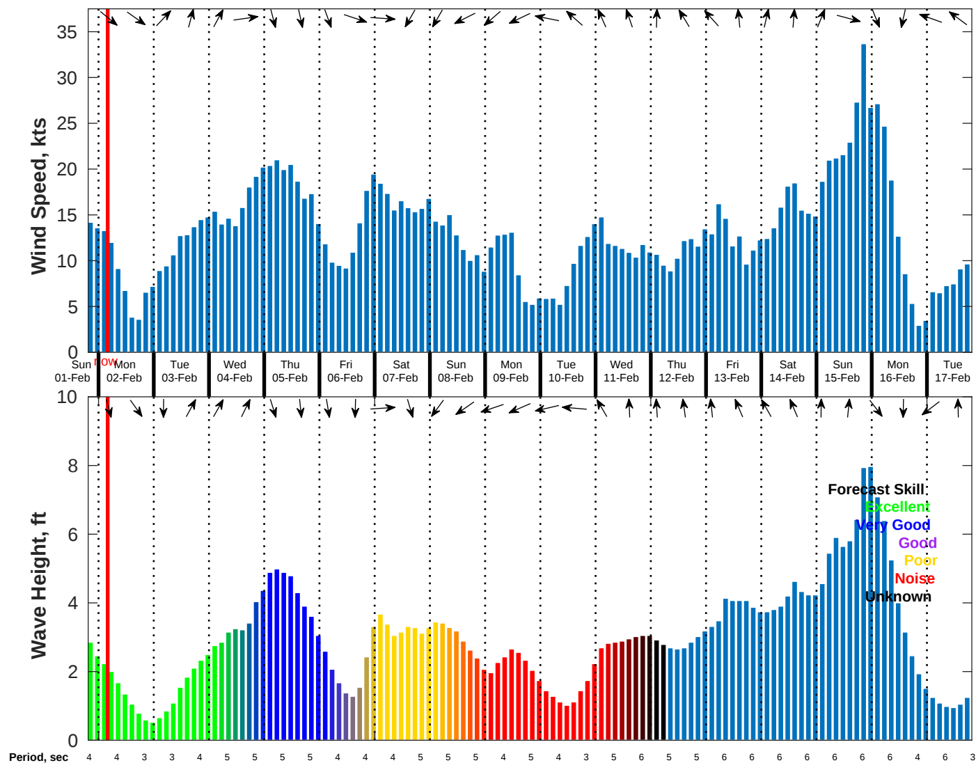
Wind & Wave Forecast for NDBC 42040 from 01-Feb-2026 19:00:00 to 17-Feb-2026 19:00:00
