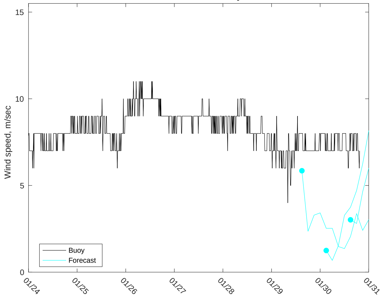
NDBC 42058 vs GFS Winds: 5 to 7 day forecast
