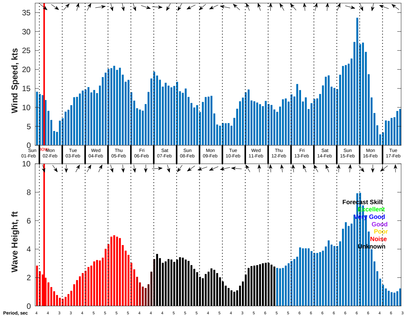
Wind & Wave Forecast for NDBC 42058 from 01-Feb-2026 20:00:00 to 17-Feb-2026 20:00:00
