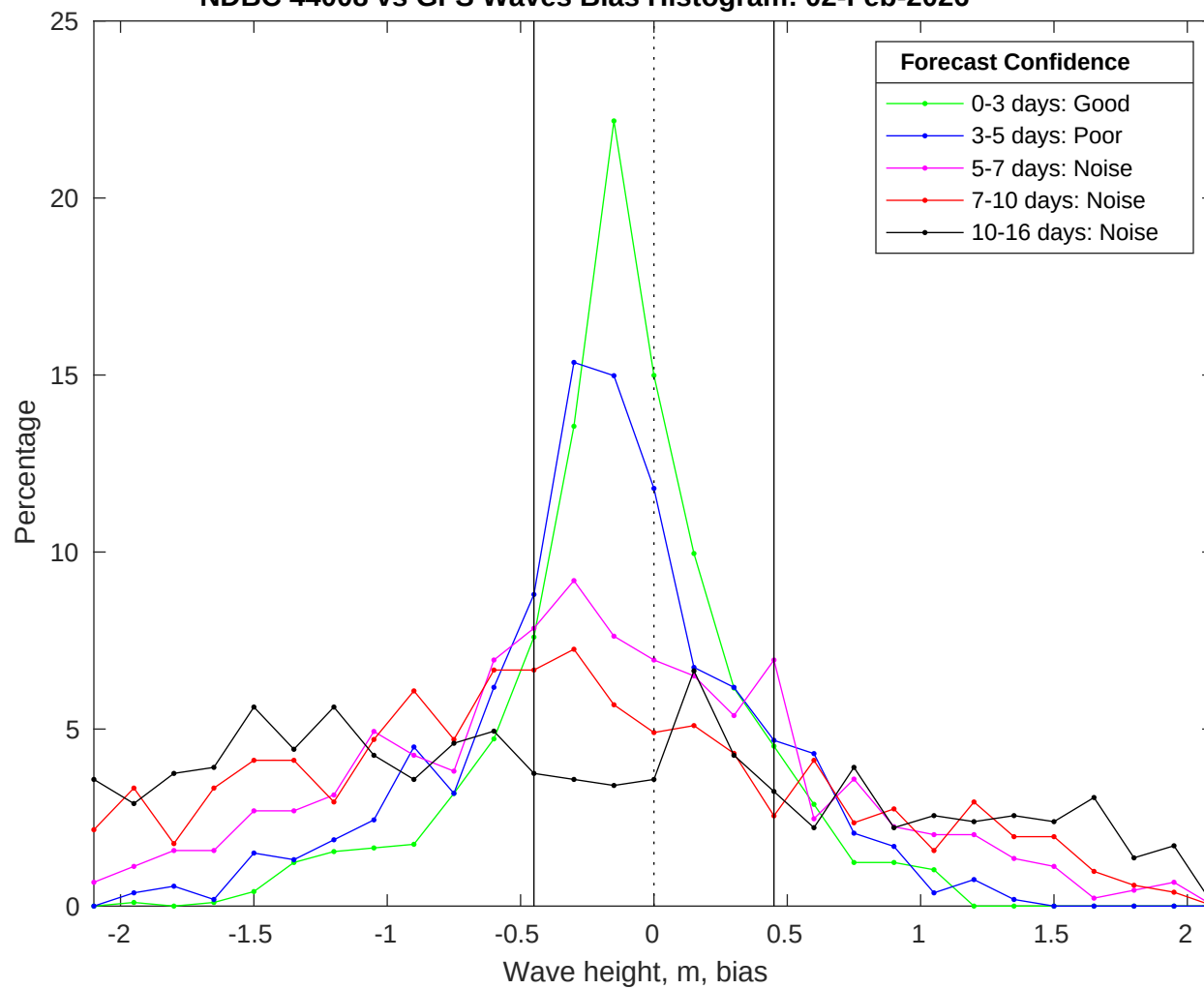
NDBC 44008 vs GFS Waves Bias Histogram: 02-Feb-2026
