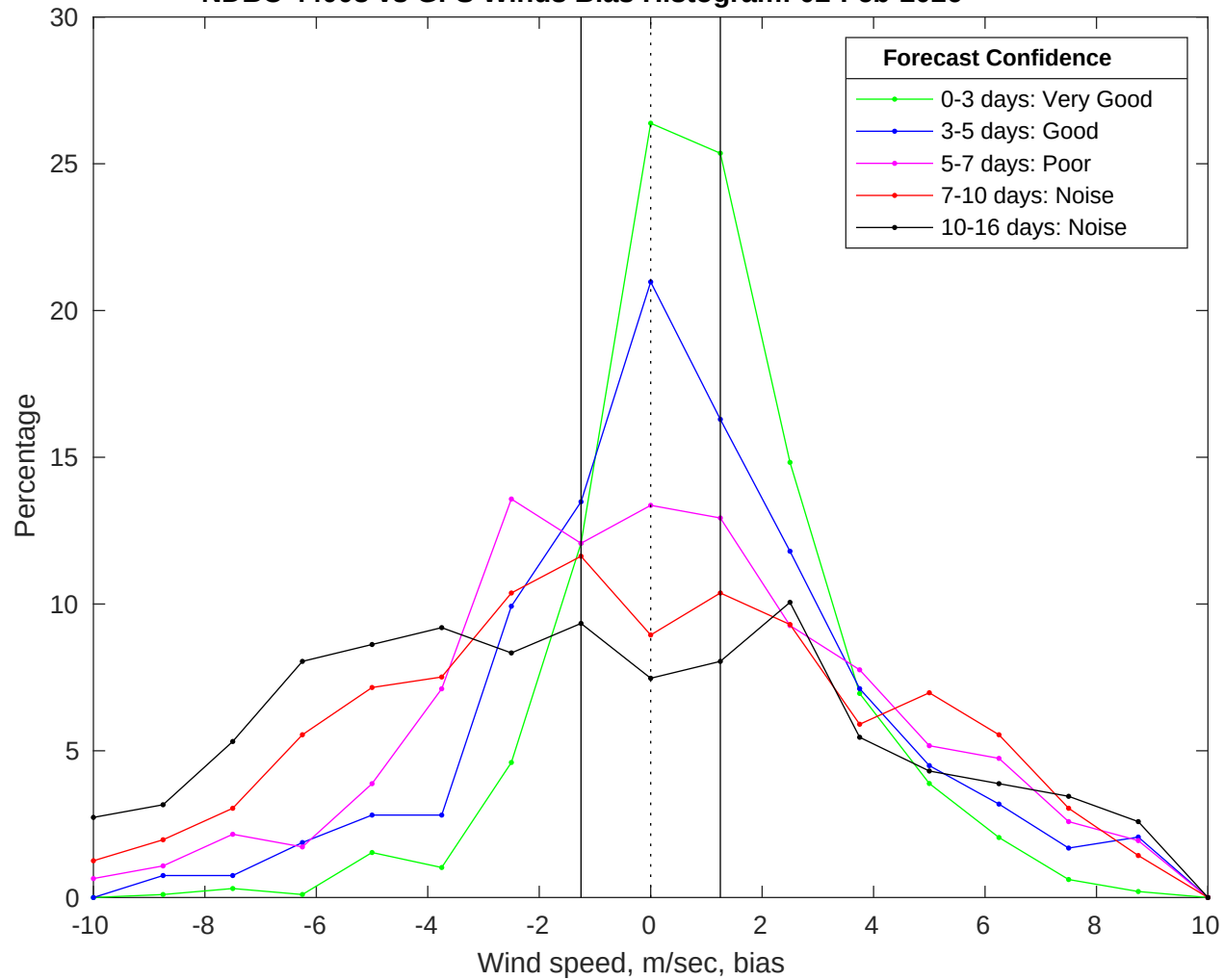
NDBC 44008 vs GFS Winds Bias Histogram: 02-Feb-2026
