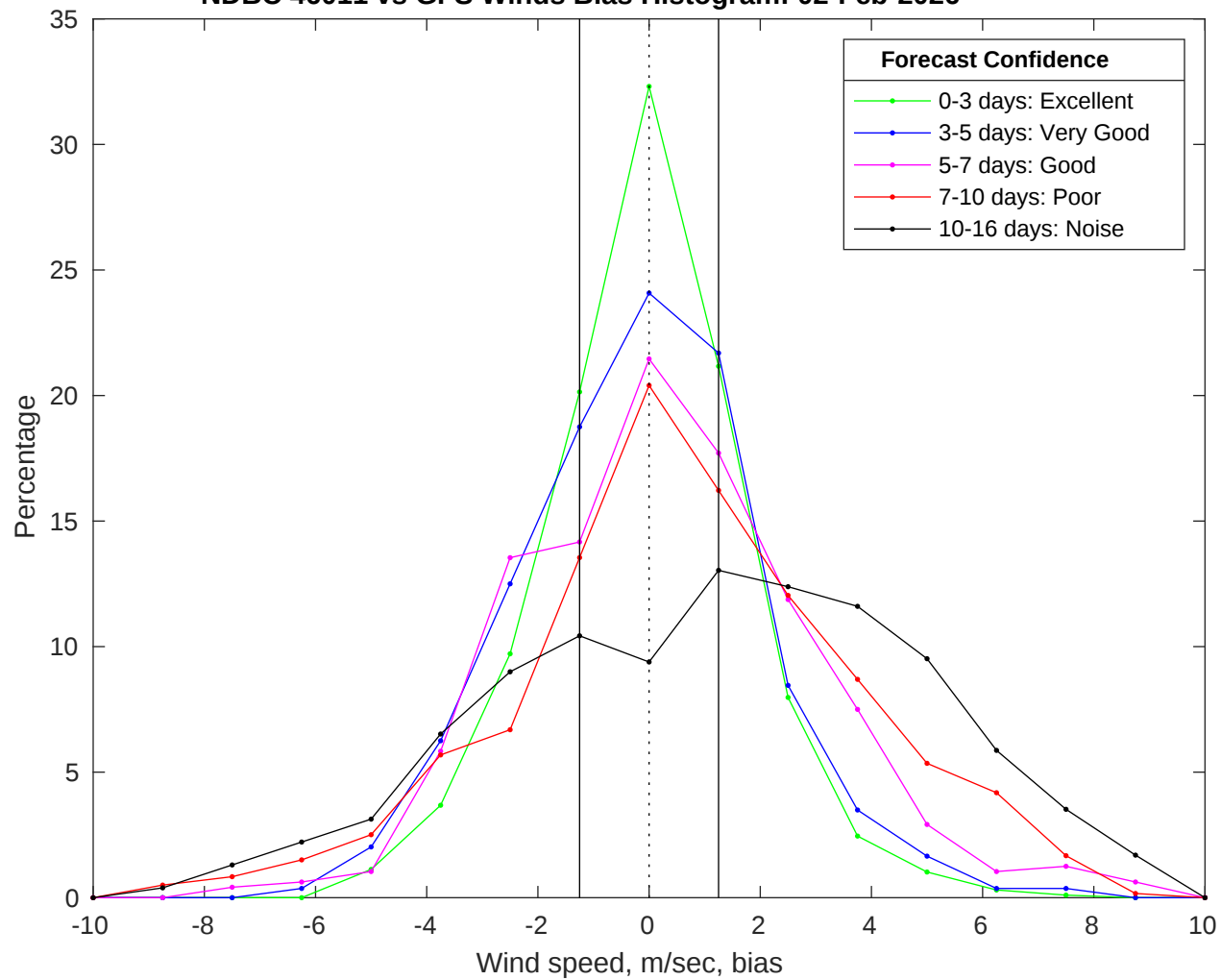
NDBC 46011 vs GFS Winds Bias Histogram: 02-Feb-2026
