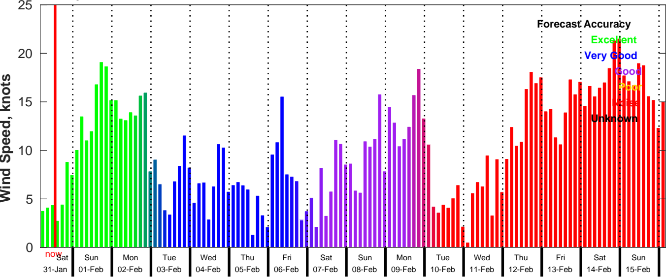
GFS Wind Speed Forecast for NDBC 46011 from 31-Jan-2026 04:00:00 to 16-Feb-2026 04:00:00
