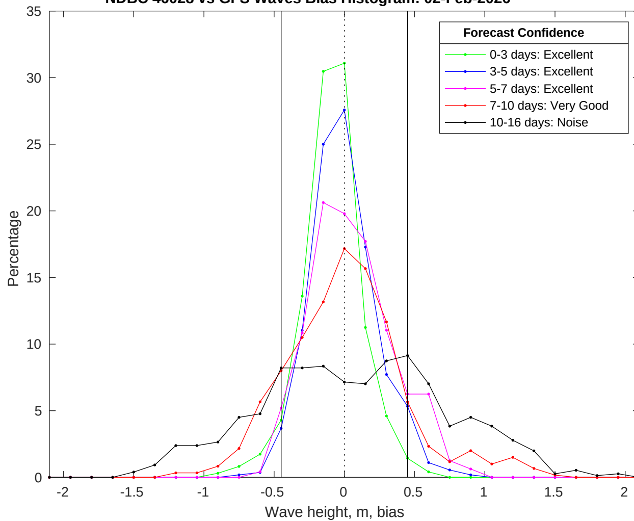
NDBC 46028 vs GFS Waves Bias Histogram: 02-Feb-2026
