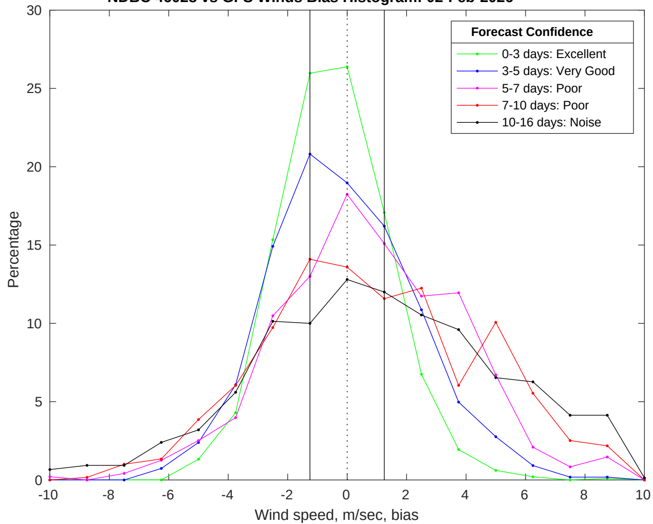
NDBC 46028 vs GFS Winds Bias Histogram: 02-Feb-2026
