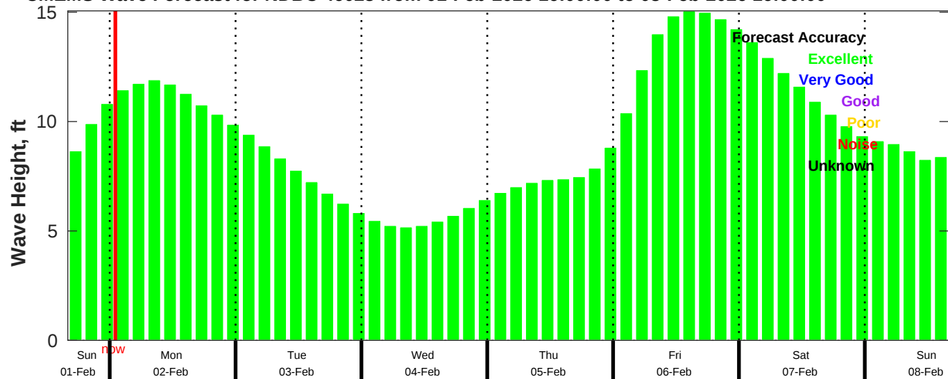
CMEMS Wave Forecast for NDBC 46028 from 01-Feb-2026 16:00:00 to 08-Feb-2026 16:00:00
