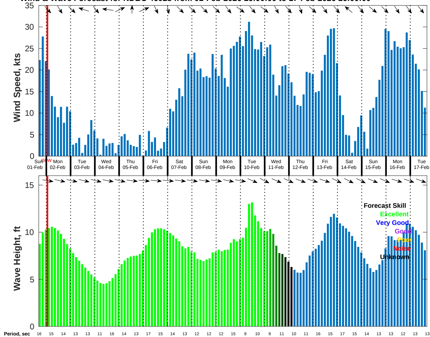
Wind & Wave Forecast for NDBC 46028 from 01-Feb-2026 16:00:00 to 17-Feb-2026 16:00:00
