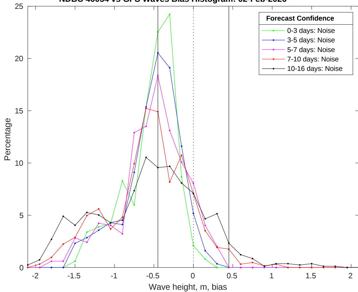
NDBC 46054 vs GFS Waves Bias Histogram: 02-Feb-2026
